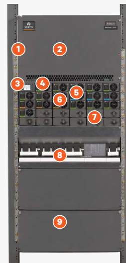
Hybrid NetSure™ 5100 Series, 28.8 kW, 23" Rack with 2 Row Distribution
